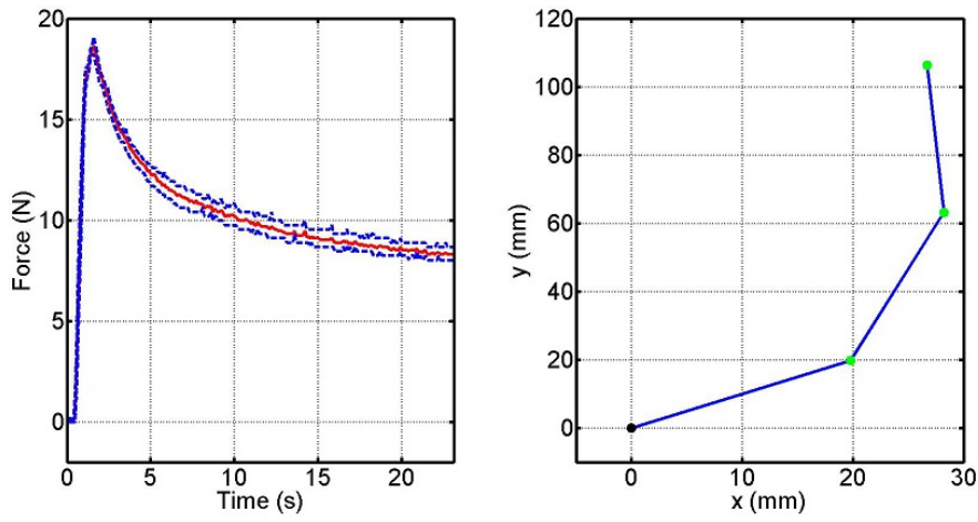
Figure 7: Force exertion for the 30% flexed configuration.
