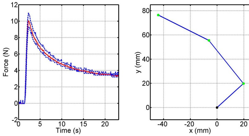
Figure 8: Force exertion for the 70% flexed configuration.
